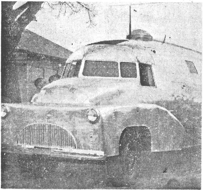
FROM CRASH TO CARAVAN: A former RAAF man, Mr Jack Fawcett, of Ramsgate (NSW), goes for a spin in his unconventional caravan, built from a crashed Dakota aircraft.
